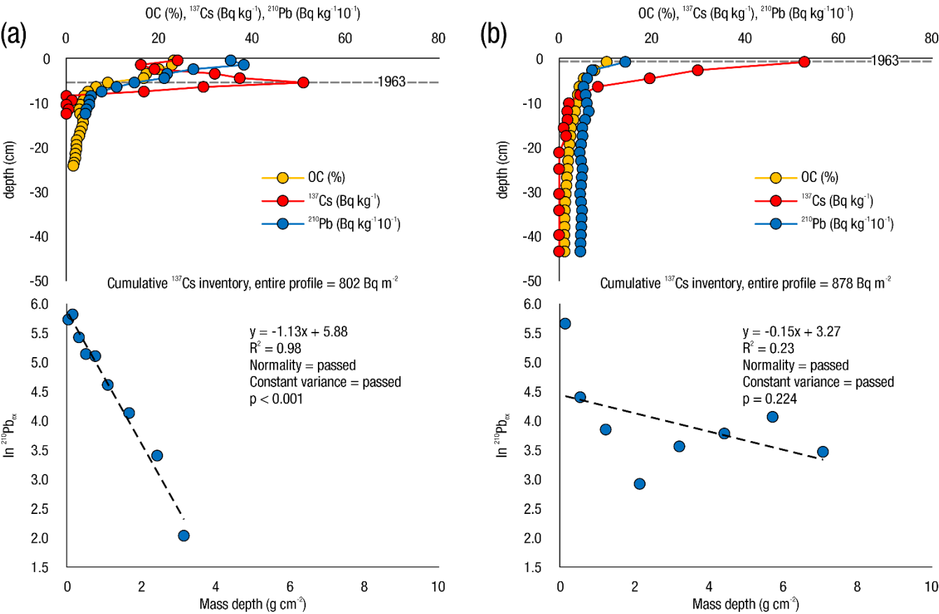
312 313 Figure 3: Examples of ^{137}\text{Cs} and ^{210}\text{Pb} classifications showing OC (%), ^{137}\text{Cs} (Bq kg ^{-1} ), and ^{210}\text{Pb} (Bq kg ^{-1} ) depth profiles and plots 314 of log-transformed ^{210}\text{Pb}_{\text{ex}} against mass depth (g cm ^{-2} ): (a) high-quality ^{137}\text{Cs} and high-quality ^{210}\text{Pb} (S-LO-I-W3-T1-CW-R1); (b) 315 high-quality ^{137}\text{Cs} and low-quality ^{210}\text{Pb} (M-OA-I-W4-T3-CW-R3).
